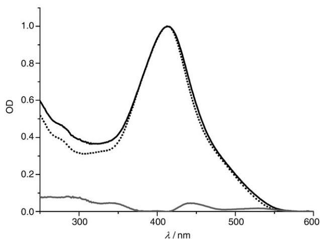
Figure 3. Normalized absorption spectra of catenane 12 (solid black line) in comparison to that of macrocycle 8 (dotted line) in dichloromethane and a difference spectrum comparing the two compounds (gray line).
