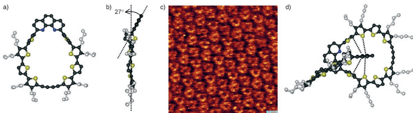
Figure 2. Calculated minimum energy conformation of macrocycle 8 (a: top view, b: side view). STM image of a monolayer of 8 at the solid (highly ordered pyrolytic graphite; HOPG)/liquid (1,2,4-trichlorobenzene) interface (c). Calculated minimum energy conformation of catenane 12 (d). The dashed lines illustrate “intermolecular” donor–acceptor interactions.
