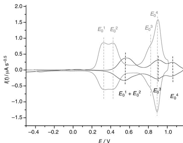
Figure 4. Deconvoluted cyclic voltammogram of catenane 12 (black line) in comparison to that of macrocycle 8 (gray line) ( 12 : 2.5 \times 10^{-4} M, 8 : 5 \times 10^{-4} M, in \text{CH}_2\text{Cl}_2/0.1 M TBAPF 6 at 295 K, \nu = 100 mVs -1 , potentials versus the ferrocene/ferrocenium (Fc/Fc + ) couple. TBA = tetrabutylammonium).
