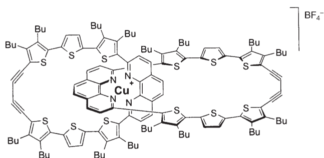
Scheme 1. Conjugated Cu I catenate synthesized from terthienylphenanthrolines.
