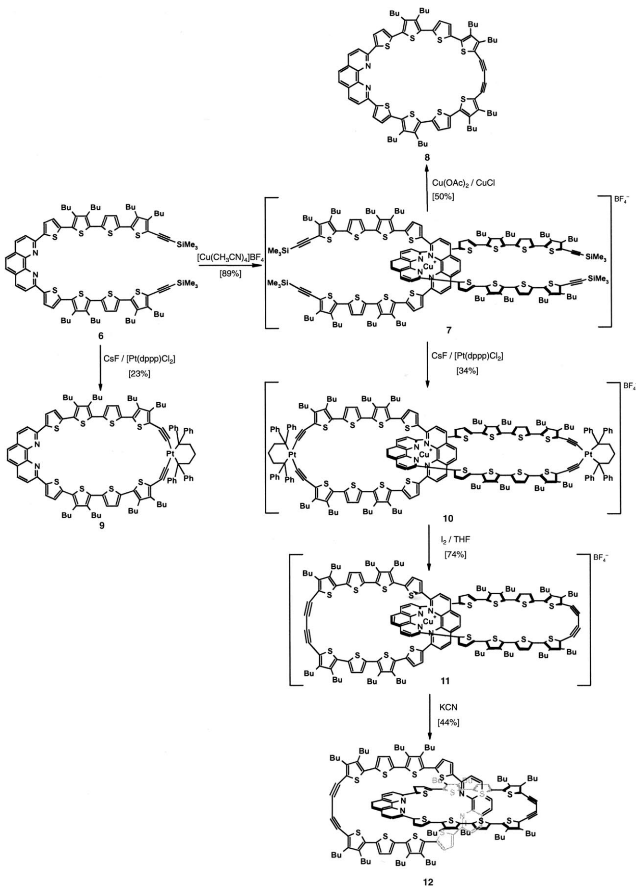
Scheme 3. 2,9-Bis(quarterthienyl)phenanthroline 6 leads to homoleptic Cu I complex 7 which can be used as a central building block for the synthesis of macrocycle 8 and catenane 12 . dppp = propane-1,3-diylbis(diphenylphosphane).
