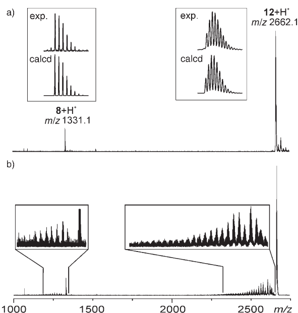
Figure 1. a) ESI-FTICR mass spectrum of a solution of catenane 12 in methanol (0.5% CF_3CO_2H ). Insets: experimental and calculated isotope patterns. b) Collision-induced dissociation (collision gas: Ar) experiment conducted with mass-selected [12+H^+] .
