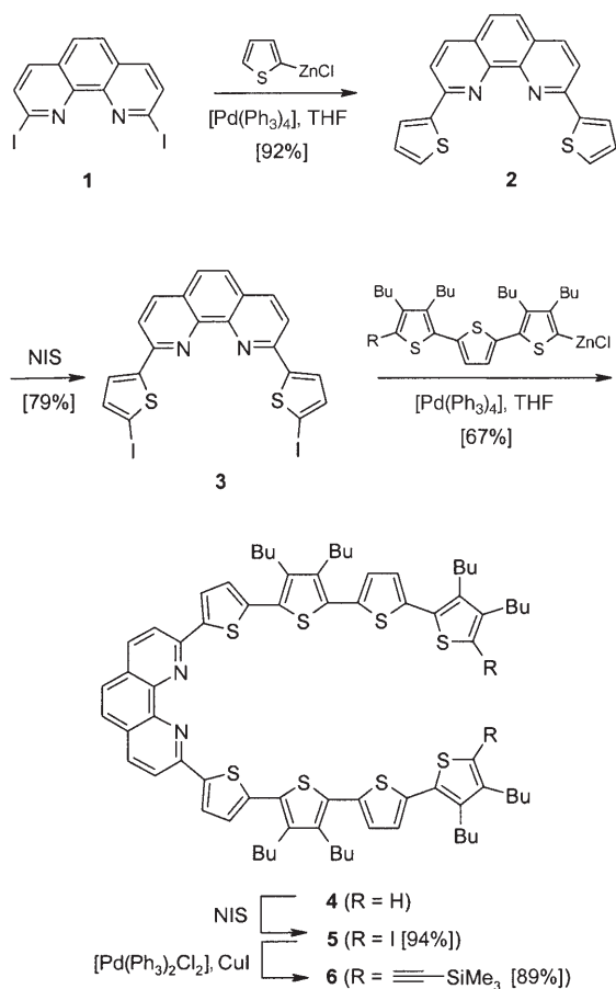
Scheme 2. Reaction sequence leading to crescent-shaped 2,9-bis-(quaterthienyl)phenanthroline ( 6 ) by Negishi-type couplings, selective iodinations, and Sonogashira–Hagihara coupling. NIS = N -iodosuccinimide.
